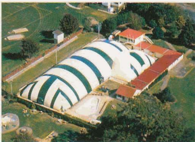
STRUCTURFLEX, AUCKLAND, N.Z. MASSEY PARK AIR SUPPORTED STRUCTURE.
